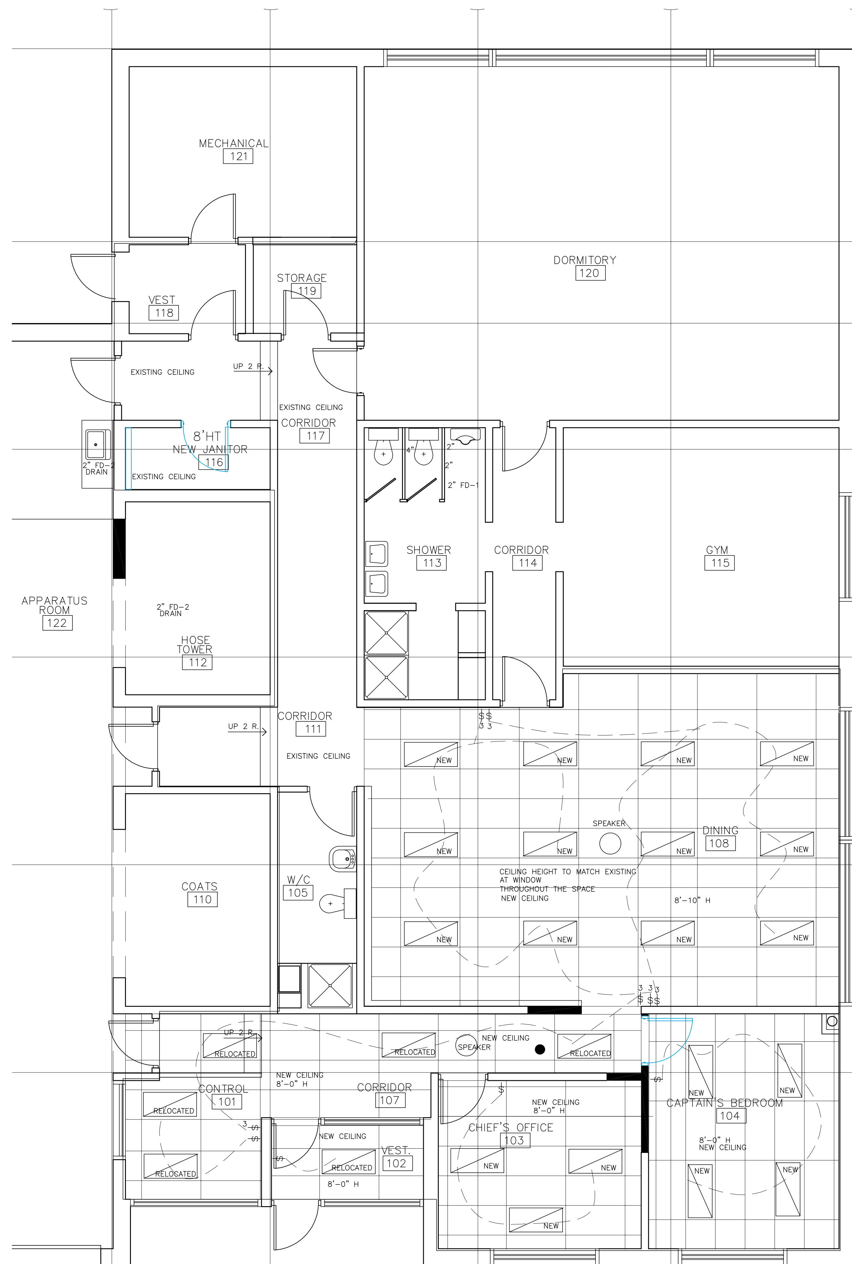
REFLECTED CEILING PLAN
